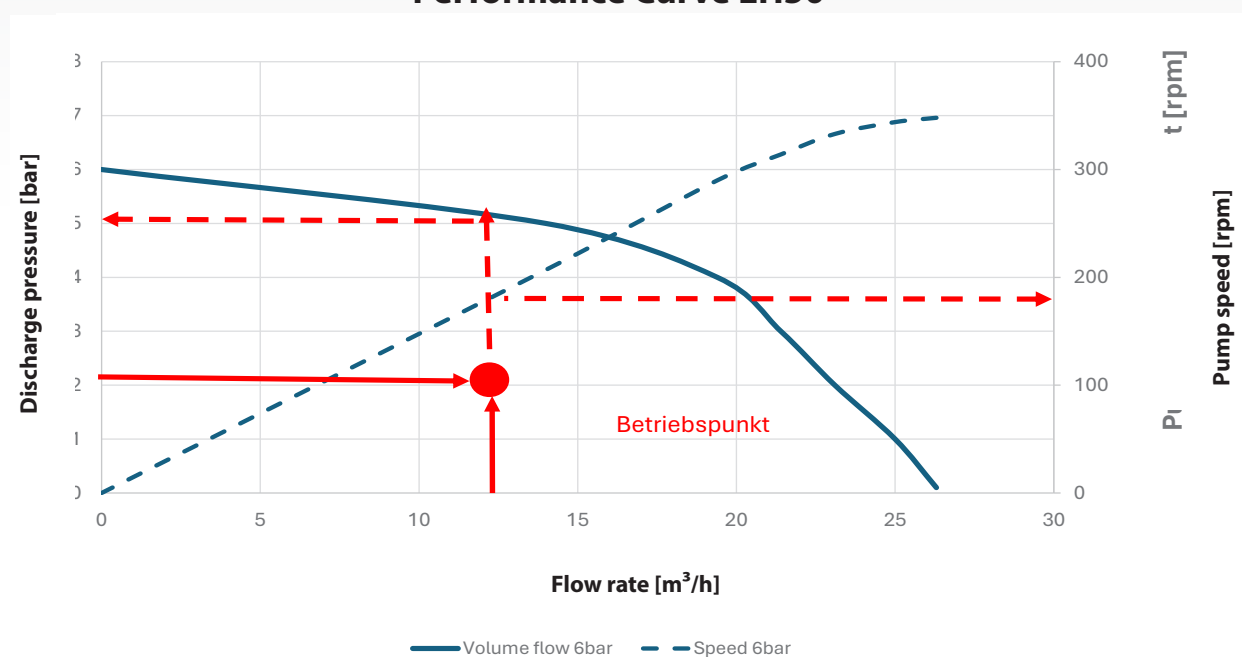
Performance Curve EH50
